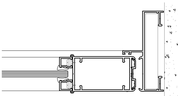
Corte 11"-11"
